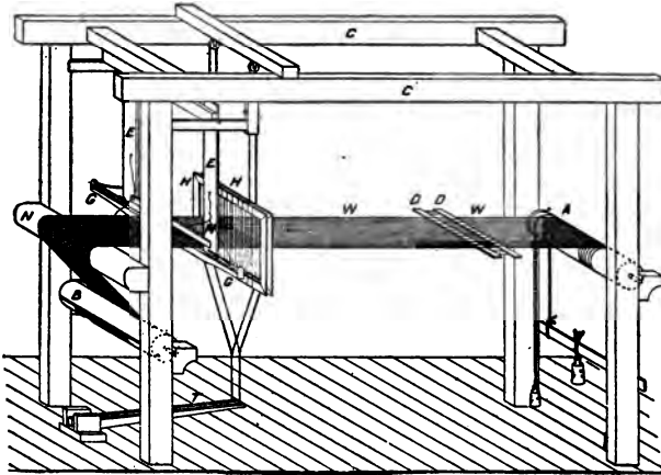
DIAGRAM OF A HAND LOOM
